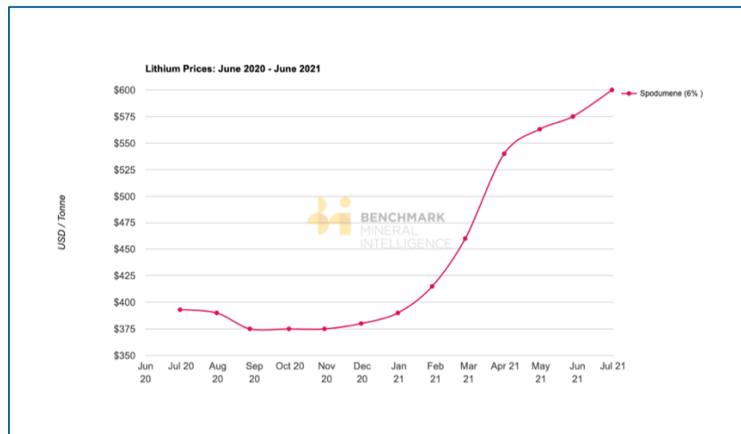
Figure 13: Chemical Grade Spodumene FOB Australia
