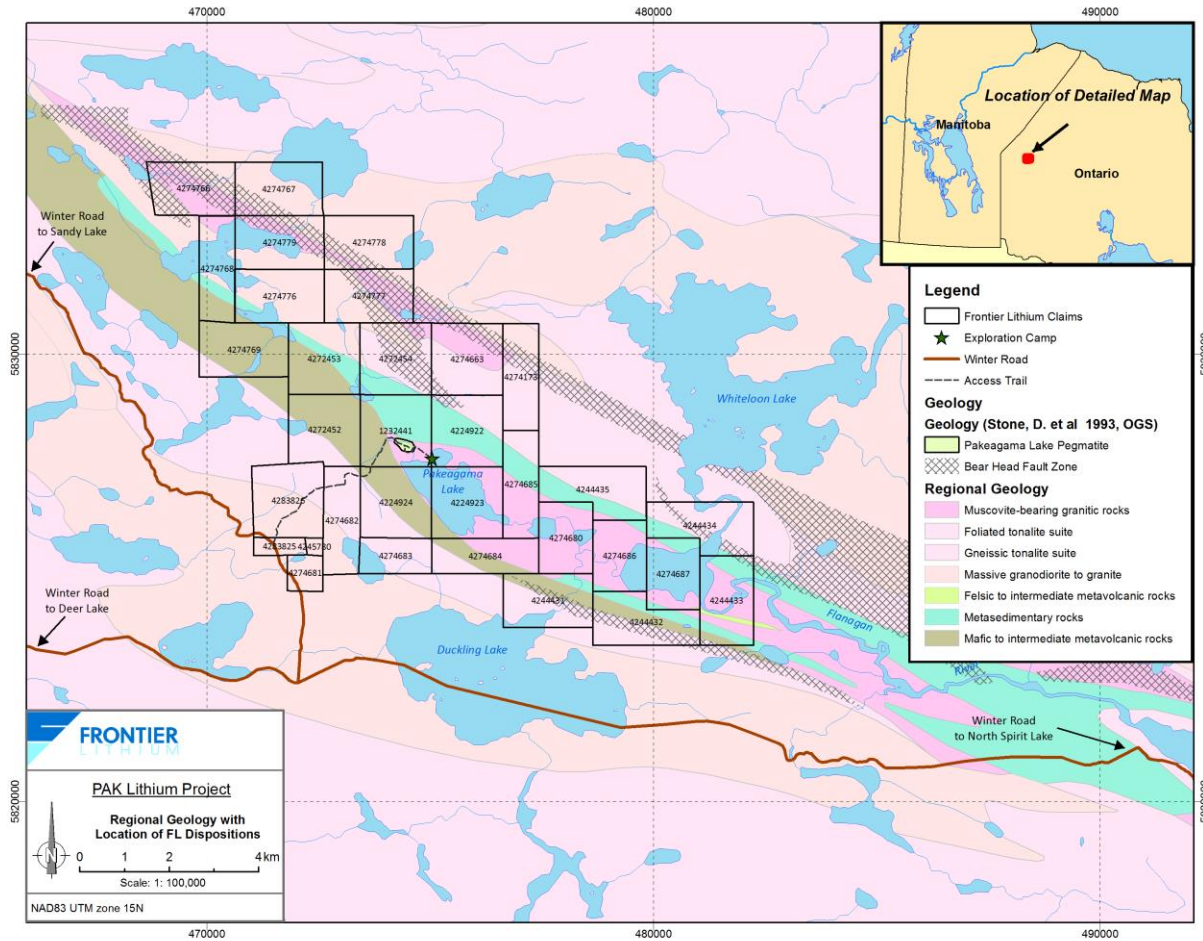
Figure II: Project Regional Geology
